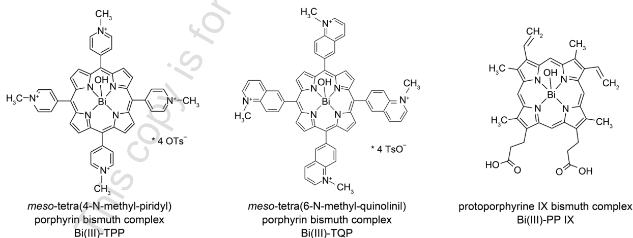
Fig. 1. Porphyrins bismuth complexes, used in the study
